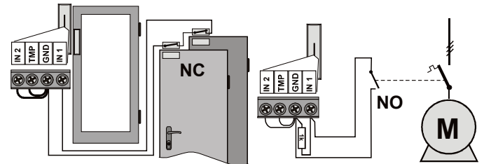
Wiring example for NC ... and NO contacts
