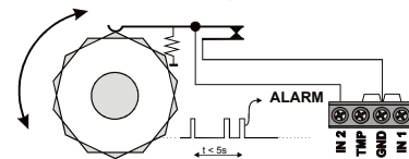
Ratchet-wheel function scheme
